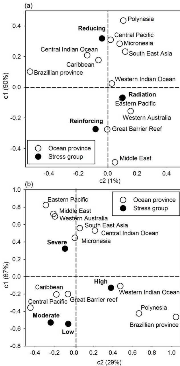
Figure 3. Correspondence bi-plots of the oceanic provinces based on the three stress groups (radiation, reducing, and reinforcing) and based on exposure severity class (a & b respectively).
